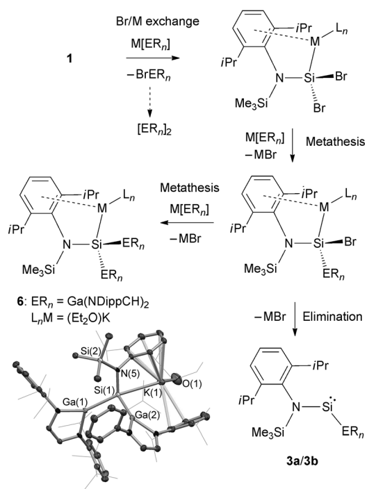
Scheme 3. Proposed mechanism for the one-pot formation of acyclic silylenes 3a and 3b from 1 through silylenoid intermediates ( M = \text{Li} or \text{K} ), and the structure of the digallylsilylenoid 6 . Key bond lengths [ \text{\AA} ] and angles [ ^\circ ]: \text{Si}(1)\text{--N}(5) 1.815(3), \text{Si}(1)\text{--Ga}(1) 2.438(1), \text{Si}(1)\text{--Ga}(2) 2.452(1), \text{Si}(1)\cdots\text{K}(1) 3.470(1); \text{N}(5)\text{--Si}(1)\text{--Ga}(1) 110.3(1), \text{N}(5)\text{--Si}(1)\text{--Ga}(2) 108.8(1), \text{Ga}(1)\text{--Si}(1)\text{--Ga}(2) 91.8(1), \text{K}(1)\text{--Si}(1)\text{--Ga}(1) 152.9(1), \text{K}(1)\text{--Si}(1)\text{--Ga}(2) 99.5(1), \text{K}(1)\text{--Si}(1)\text{--N}(5) 89.3(1).
